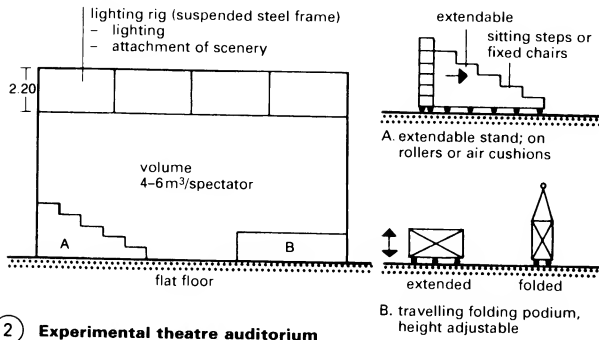
② Experimental theatre auditorium
